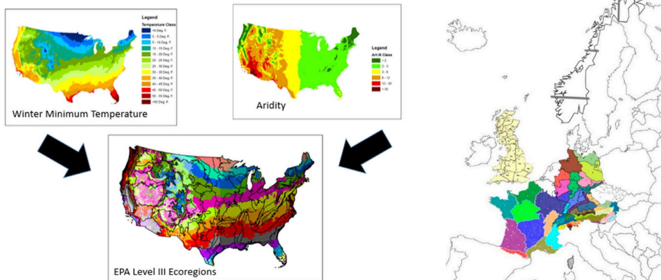
Figure 3. Seed zones in the United States and Europe: Left: U.S. provisional seed zones for native plants (color polygons) are unique, climatically delineated (temperature-aridity) areas nested within EPA Level III Ecoregion boundaries (black lines). The provisional zones can be used to guide seed sourcing decisions when species-specific genetic information is lacking (Bower et al. 2014). Right: National seed zones developed for European countries (De Vitis et al. 2017). Permission provided.
